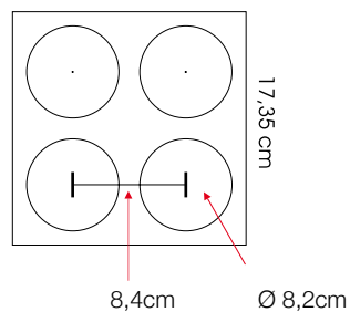
Opening in the ceiling
