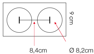
Opening in the ceiling
